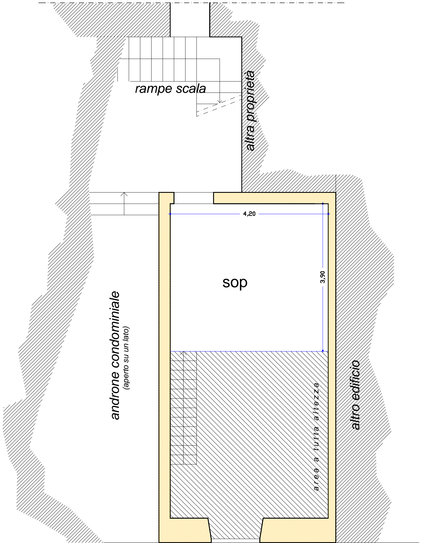
pianta piano soppalco
